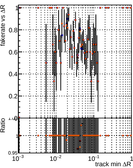
Fake rate vs \Delta R(\text{track, jet}) Legend: original (black) noPU (blue) paretofront (red) MaxEffOnly (green) MinHitOnly (orange) MaxHitOnly-FW2 (purple)
