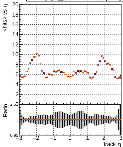
mean hits vs \eta DQM_TT original_noPU DQM_TT paretofrontMaxEffOnlyFWD2_PU DQM_TT paretofrontMinFWD2_PU DQM_TT paretofrontMaxHitsOnlyFWD2_PU
