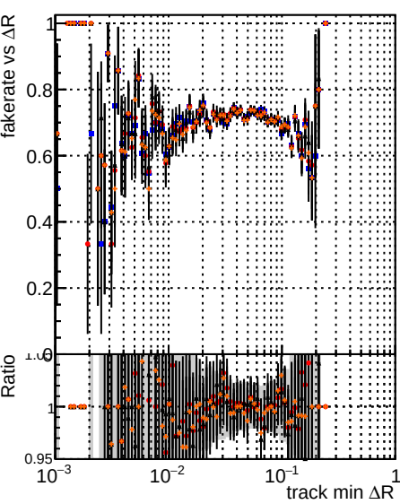
Fake rate vs \Delta R(\text{track, jet}) Legend: original noPU (black line) paretofrontMaxEffOnlyFWD2_PU (blue line) paretofrontMinHitOnlyFWD2_PU (red line) paretofrontMaxHitOnlyFWD2_PU (orange line)
