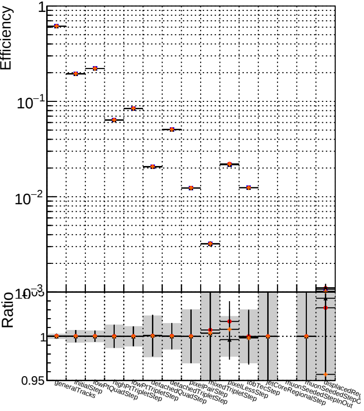
DQM_TT_original_noPU DQM_TT_paretofrontMaxEffOnlyFWD_PU DQM_TT_paretofrontMinFROnlyFWD_PU DQM_TT_paretofrontMaxHitsOnlyFWD_PU
