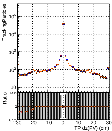
N of simulated tracks vs dz(PV) 10000 5000 2500 1000 500 250 100 50 25 10 5 2 1
