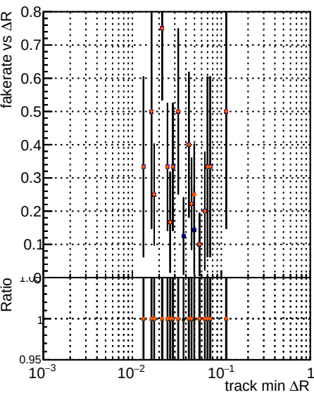
Fake rate vs ΔR(track, jet) Legend: DOM (black line) TT (blue line) original (red line) noPU (orange line) paretofrontMaxEffOnlyFWD_PU (black line with dots) paretofrontMinEffOnlyFWD_PU (black line with dots) paretofrontMaxHitOnlyFWD_PU (black line with dots)
