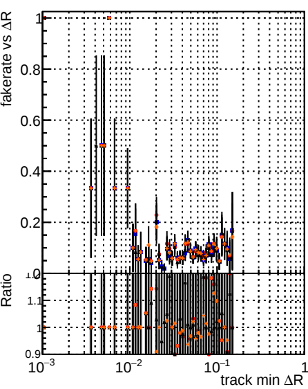
Fake rate vs \Delta R(\text{track, jet}) Legend: original (black) noPU (blue) paretofront (red) MinEffOnlyFWD_PU (green) MinHitOnlyFWD_PU (orange) MaxHitOnlyFWD_PU (purple)
