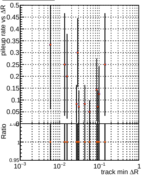
Fake rate vs ΔR(track, jet) | Duplicates Rate vs ΔR(track, jet) | Pileup rate vs ΔR(track, jet) Legend: original noPU paretofrontMaxEffOnlyFWD_PU paretofrontMinHitOnlyFWD_PU paretofrontMaxHitOnlyFWD_PU
