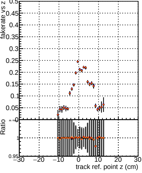
Fake rate vs verpos Legend: original noPU paretofrontMaxEffOnlyFWD_PU paretofrontMinEffOnlyFWD_PU paretofrontMaxHitOnlyFWD_PU
