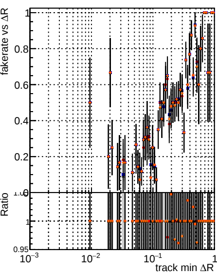
Fake rate vs ΔR(track, jet) Legend: DOM (black) TT (blue) original (red) noPU (green) paretofront (grey) MaxEffOnlyFWD_PU (orange) MinHitOnlyFWD_PU (purple) paretofrontMaxHitOnlyFWD_PU (brown)
