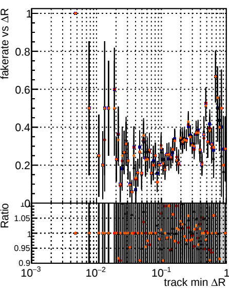
Fake rate vs \Delta R(\text{track, jet}) Legend: DOM (black) TT (blue) original (red) noPU (green) paretofrontMaxEffOnlyFWD_PU (orange) paretofrontMinHitOnlyFWD_PU (purple) paretofrontMaxHitOnlyFWD_PU (brown)
