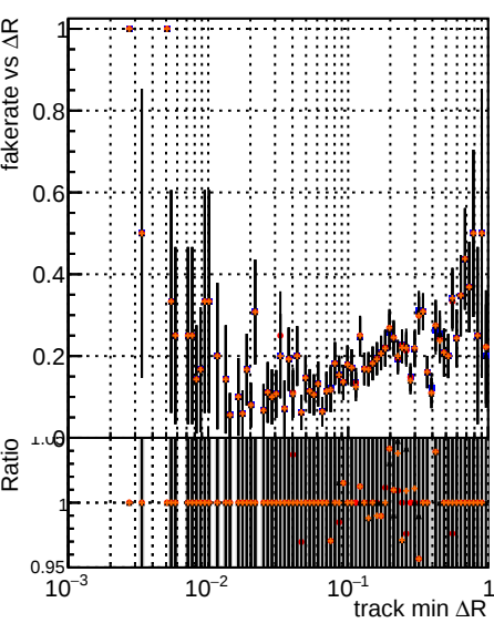
Fake rate vs \Delta R(\text{track, jet}) Legend: DOM (black line) TT (blue line) original (red line) noPU (orange line) paretofrontMinEffOnlyFWD_PU (black line with dots) paretofrontMinHitOnlyFWD_PU (black line with dots) paretofrontMaxHitOnlyFWD_PU (black line with dots)
