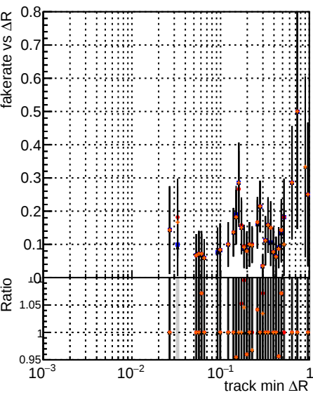
Fake rate vs ΔR(track, jet) | Duplicates Rate vs ΔR(track, jet) | Pileup rate vs ΔR(track, jet) Legend: DOM TT original no PU DOM TT paretofrontMaxEffOnlyFWD_PU DOM TT paretofrontMinHitOnlyFWD_PU DOM TT paretofrontMaxHitOnlyFWD_PU
