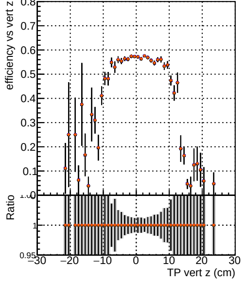
Efficiency vs vert z —●— DOM TT original noPU —●— DOM TT paretofrontMaxEffOnlyFWD_PU —●— DOM TT paretofrontMinFROnlyFWD_PU —●— DOM TT paretofrontMaxHitsOnlyFWD_PU
