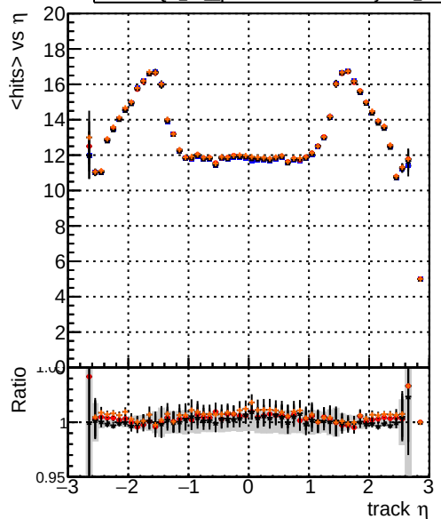
mean hits vs \eta Legend: - DQM_TT original noPU - DQM_TT paretofrontMaxEffOnlyFWD_PU - DQM_TT paretofrontMinFROnlyFWD_PU - DQM_TT paretofrontMaxHitsOnlyFWD_PU
