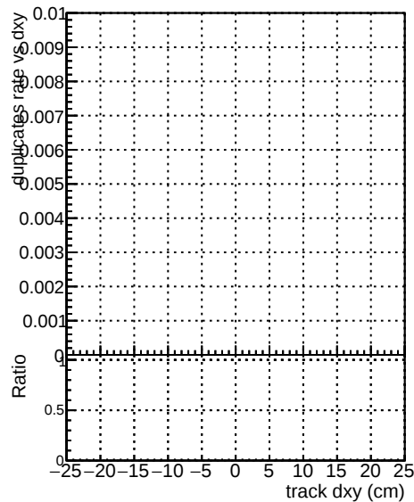
\text{FWD} = \text{PU}
