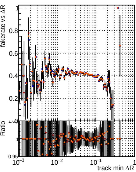
Fake rate vs \Delta R(\text{track, jet}) Legend: original (black) noPU (blue) paretofront (red) MaxEffOnlyFWD_PU (green) MinHitOnlyFWD_PU (orange) HitOnlyFWD_PU (yellow)
