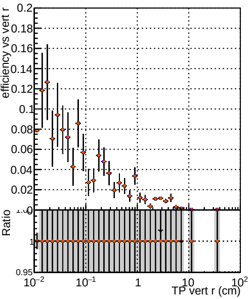
Efficiency vs vertpos —●— DQM TT original noPU —●— DQM TT paretofrontMaxEffOnlyFB2_PU —●— DQM TT paretofrontMinFROnlyFB2_PU —●— DQM TT paretofrontMaxHitsOnlyFB2_PU
