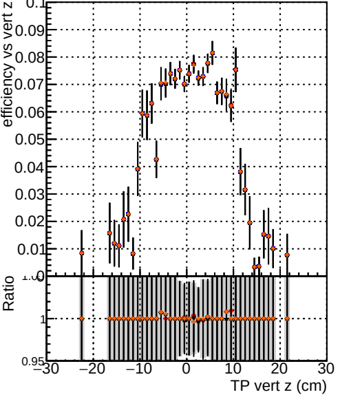
Efficiency vs vertpos —●— DQM TT original noPU —●— DQM TT paretofrontMaxEffOnlyFB2_PU —●— DQM TT paretofrontMinFROnlyFB2_PU —●— DQM TT paretofrontMaxHitsOnlyFB2_PU
