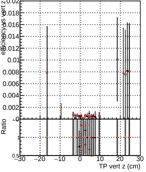
Efficiency vs TP vert z (cm) —●— DQM TT original noPU —◆— DQM TT paretofrontMaxEffOnlyFB2_PU —▲— DQM TT paretofrontMinF0OnlyFB2_PU —■— DQM TT paretofrontMaxHitsOnlyFB2_PU
