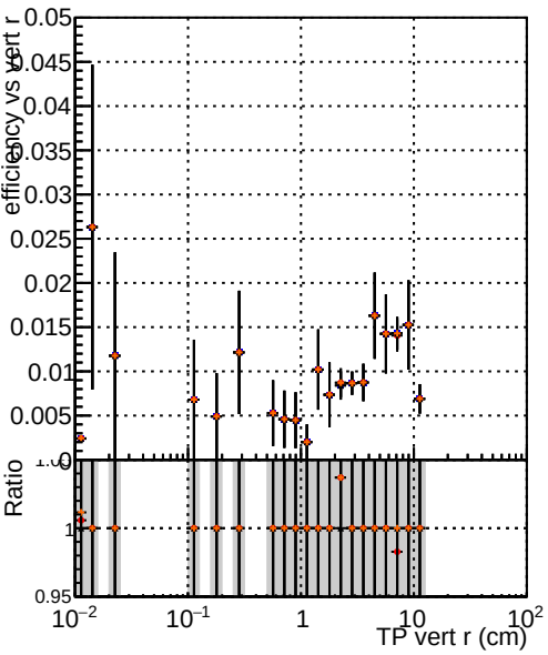
Efficiency vs TP vert r (cm) —●— DQM TT original noPU —●— DQM TT paretofrontMaxEffOnlyFB2_PU —●— DQM TT paretofrontMinFROnlyFB2_PU —●— DQM TT paretofrontMaxHitsOnlyFB2_PU
