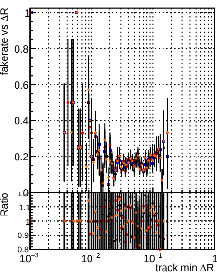
Fake rate vs \Delta R(\text{track, jet}) Legend: DOM TT original no PU DOM TT paretofrontMaxEffOnlyFB2_PU DOM TT paretofrontMinHitOnlyFB2_PU DOM TT paretofrontMaxHitOnlyFB2_PU
