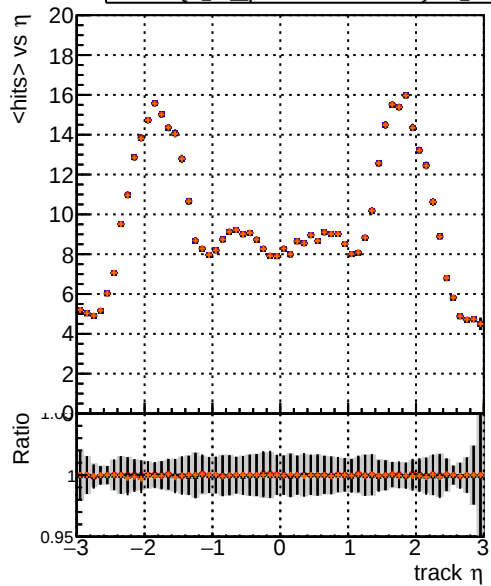
mean hits vs \eta Legend: - DQM_TT original noPU - DQM_TT paretofrontMaxEffOnlyFB2_PU - DQM_TT paretofrontMinFitsOnlyFB2_PU - DQM_TT paretofrontMaxHitsOnlyFB2_PU
