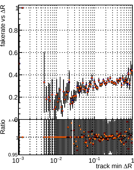
Fake rate vs \Delta R(\text{track, jet}) Legend: original noPU paretofrontMinHitOnlyFB2_PU paretofrontMaxHitOnlyFB2_PU paretofrontMinHitOnlyFB2_PU paretofrontMaxHitOnlyFB2_PU
