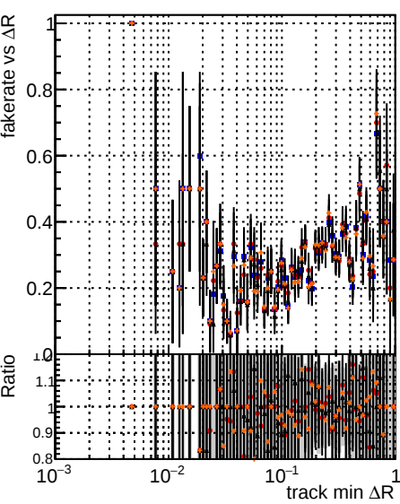
Fake rate vs \Delta R (track, jet) | Duplicates Rate vs \Delta R (track, jet) | Pileup rate vs \Delta R (track, jet) Legend: DOM (black), TT (blue), original (red), noPU (orange), paretofrontMaxEffOnlyFB2_PU (green), paretofrontMinHitOnlyFB2_PU (purple), paretofrontMaxHitOnlyFB2_PU (brown).
