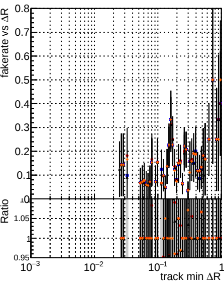
Fake rate vs \Delta R(\text{track, jet}) Legend: original noPU paretofrontMaxHitOnlyFB2_PU paretofrontMinHitOnlyFB2_PU paretofrontMaxHitOnlyFB2_PU
