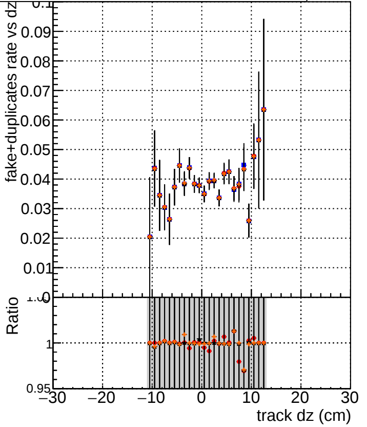
Legend: DQM_TT_original_noPU (grey square) DQM_TT_paretofrontMaxEffOnlyFB2_PU (red circle) DQM_TT_paretofrontMinFROnlyFB2_PU (black triangle) DQM_TT_paretofrontMaxHitsOnlyFB2_PU (orange circle)
