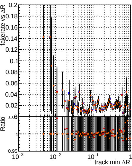
Fake rate vs \Delta R(\text{track, jet}) Legend: DOM TT original no PU DOM TT paretofrontMinEffOnlyFB2_PU DOM TT paretofrontMinHitOnlyFB2_PU DOM TT paretofrontMaxHitOnlyFB2_PU
