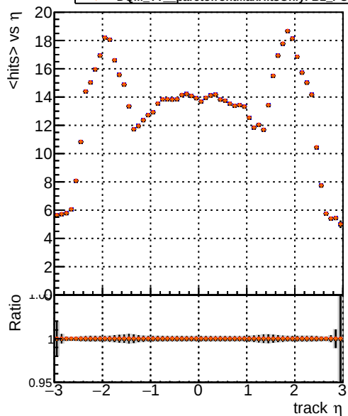
mean hits vs \eta Legend: blue line: DQM TT original noPU red line: DQM TT paretofrontMaxEffOnlyFB2_PU black line: DQM TT paretofrontMinFROnlyFB2_PU orange line: DQM TT paretofrontMaxHitsOnlyFB2_PU
