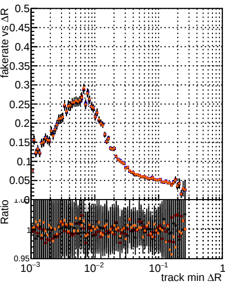
Fake rate vs \Delta R (track, jet) Legend: original noPU paretofrontMaxEffOnlyFB2_PU paretofrontMinHitOnlyFB2_PU paretofrontMaxHitOnlyFB2_PU
