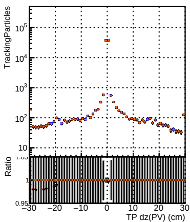
N of simulated tracks vs dz(PV) 10000 1000 100 10 1
