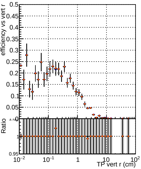
Efficiency vs TP vert r (cm) — DOM TT original noPU — DOM TT paretofrontMaxEff_PU — DOM TT paretofrontMaxHits_PU — DOM TT paretofrontMinFR_PU
