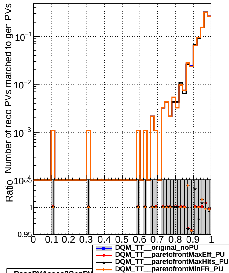
RecoPVAssoc2GenPVMatched_missing
