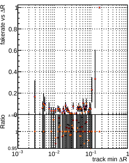
Fake rate vs \Delta R(\text{track, jet}) Legend: original noPU (black line with error bars) paretofrontMaxEff (orange dots) paretofrontMin-R (grey line with error bars)
