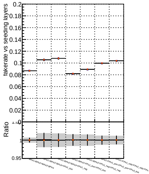
Fake rate vs. - DOM IT original noPU - DOM IT particle on Max Eff. PU - DOM IT particle on Min Eff. PU
