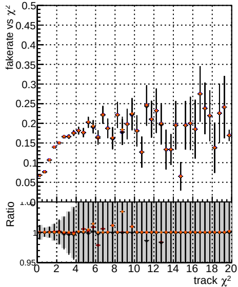
Fake rate vs. - DOM IT original noPU - DOM IT particle on Max Eff. PU - DOM IT particle on Min Eff. PU
