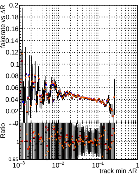
Fake rate vs \Delta R(\text{track}, \text{jet}) Legend: original noPU paretofrontMaxEff paretofrontMinR paretofrontMinR
