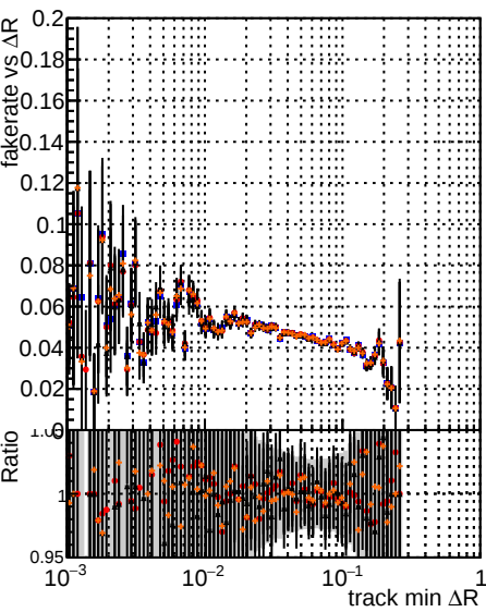
Fake rate vs \Delta R(\text{track, jet}) Legend: original noPU paretofrontMaxEff_PU paretofrontMaxHits_PU paretofrontMinR_PU
