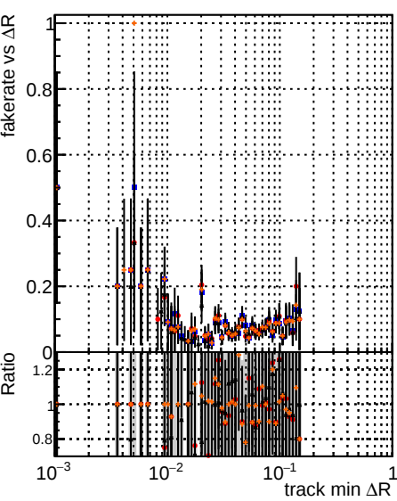
Fake rate vs \Delta R(\text{track, jet}) Legend: DOM TT original noPU DOM TT paretofrontMaxEff PU DOM TT paretofrontMinR PU
