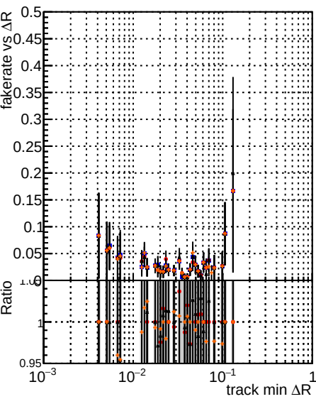
Fake rate vs \Delta R(\text{track, jet}) Legend: original noPU (black line with error bars) paretofrontMaxEff PU (orange dots) paretofrontMin-R PU (grey line with error bars)
