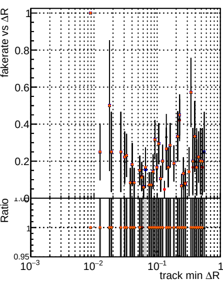
Fake rate vs \Delta R(\text{track, jet}) Legend: original noPU (black line with error bars) paretofrontMaxEff (red dots with error bars) paretofrontMin-R (orange dots with error bars)
