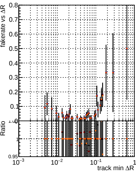
Fake rate vs \Delta R(\text{track, jet}) Legend: original noPU (black line) paretofrontMaxEff (red line) paretofrontMin-R (orange line)
