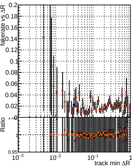
Fake rate vs \Delta R(\text{track, jet}) Legend: original noPU (black line with dots) paretofrontMaxEff PU (orange line with dots) paretofrontMin-R PU (red line with dots)
