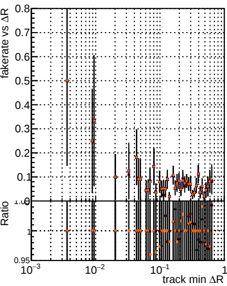
Fake rate vs ΔR(track, jet) for different PU models Model Line Style Color Symbol original no PU Solid Black None paretofrontMaxEff Dashed Blue Circle paretofrontMaxHits Dashed Red Circle paretofrontMinR Dashed Orange Circle
