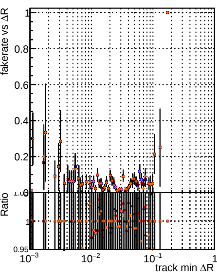
Fake rate vs \Delta R(\text{track, jet}) Legend: original noPU (black line with error bars) paretofrontMaxEff (orange dots) paretofrontMin-R (grey line with error bars) paretofrontMin-R PU (orange dots)
