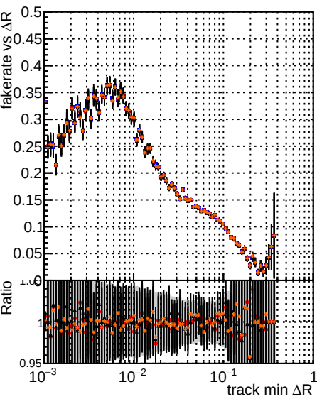
Fake rate vs \Delta R(\text{track, jet}) Legend: original (black line) noPU (blue line) ParetoFrontMaxEff (red line) ParetoFrontMinR (orange line)
