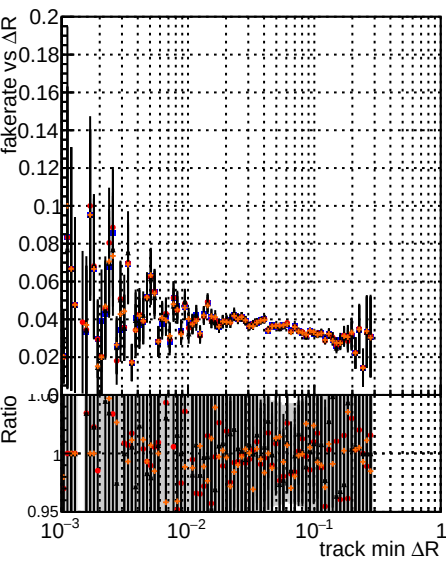
Fake rate vs \Delta R(\text{track, jet}) Legend: original (black line) frontMaxEff (blue line) frontMinEff (red line) frontMinR (orange line)
