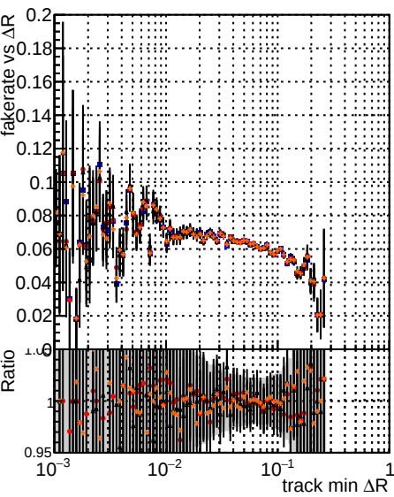
Fake rate vs \Delta R(\text{track, jet}) Legend: original noPU paretofrontMaxEff paretofrontMaxHits paretofrontMinR
