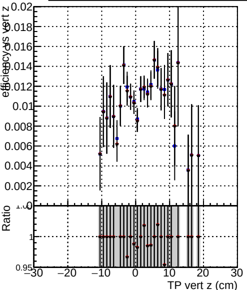
Efficiency vs TP vert z (cm) Legend: DQM_TT_original DQM_TT_initOnlyFWD0_PU DQM_TT_initOnlyFWD0_PU
