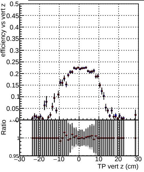
Efficiency vs vertpos DQM_TT_original DQM_TT_initOnlyFWD0_PU DQM_TT_initOnlyFWD0_PU
