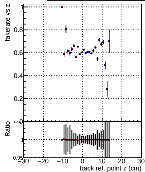
Fake rate vs verpos Legend: DOM TT original (black dots) DOM TT initOnlyFWD0 (red dots) DOM TT initOnlyFWD0 PU (black dots)
