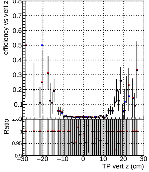
Efficiency vs. TP vert z (cm) —●— DQM_TT_original —●— DQM_TT_initOnlyFWD0_PU —●— DQM_TT_initOnlyFWD0_PU
